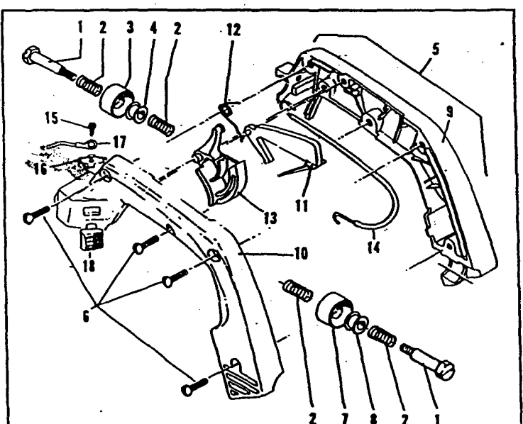
HANDLE ASSEMBLY FIGURE 4
